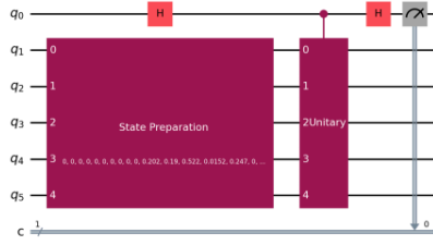
Fig. 4. Circuit diagram of the ISDO-B' implementation. The control transition unitary U_{\chi\psi} is used to estimate the linear overlap \text{Re}\langle\phi|\psi\rangle by measuring the ancilla qubit in the Z-basis.
